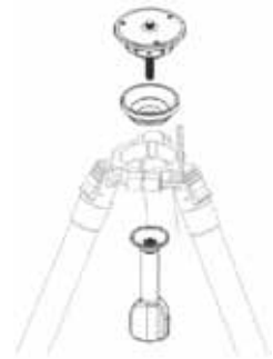
Optional bowls and leveling heads for video applications
